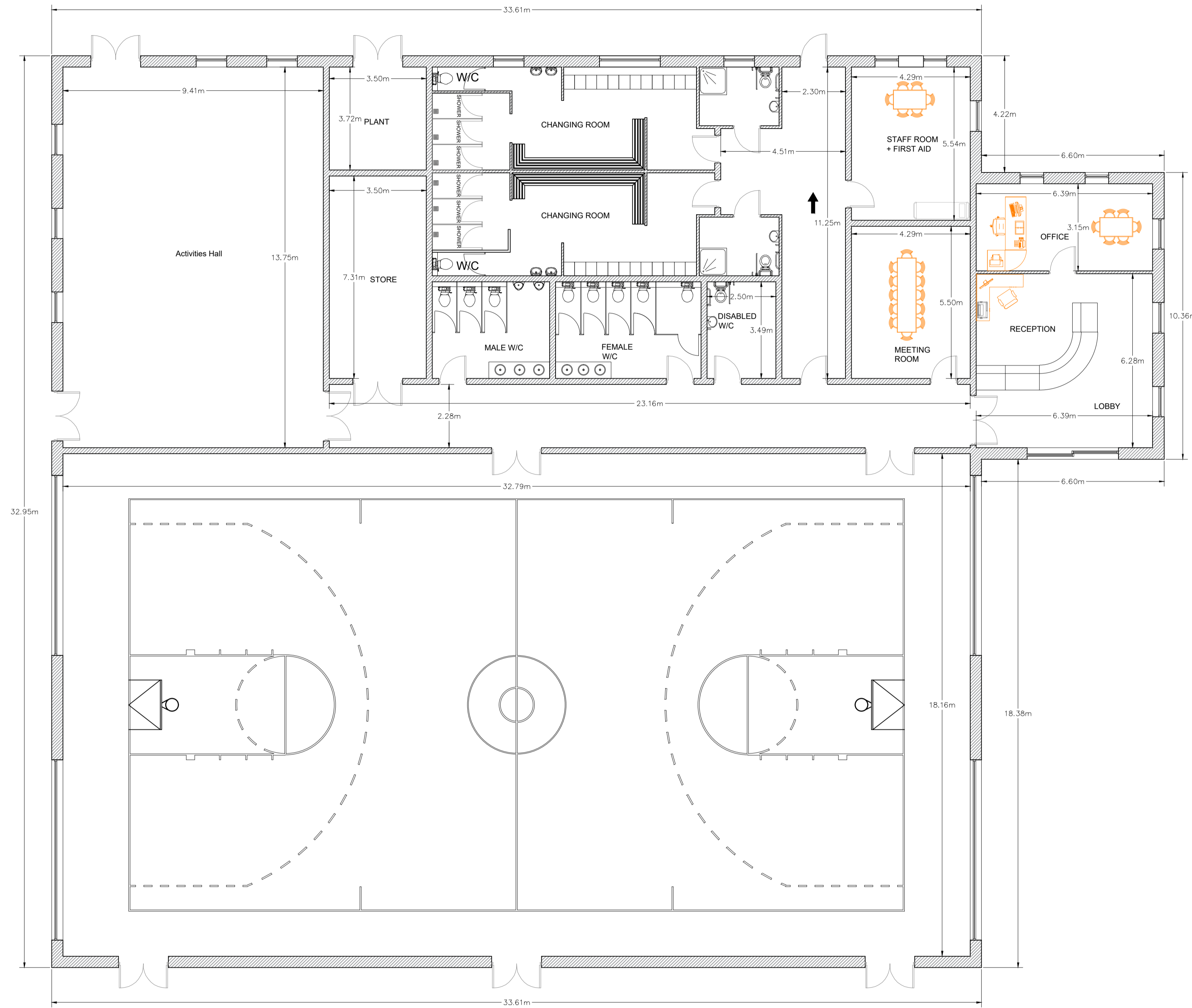
PROPOSED FLOOR PLAN
