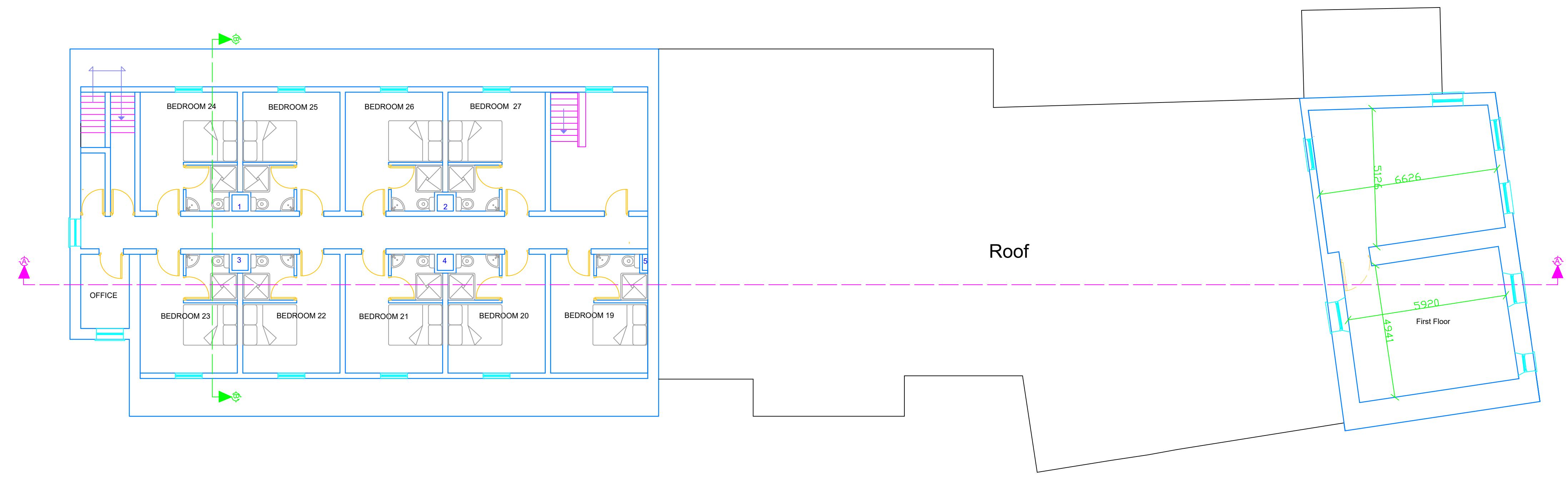
ATTIC FLOOR PLAN - EXISTING
