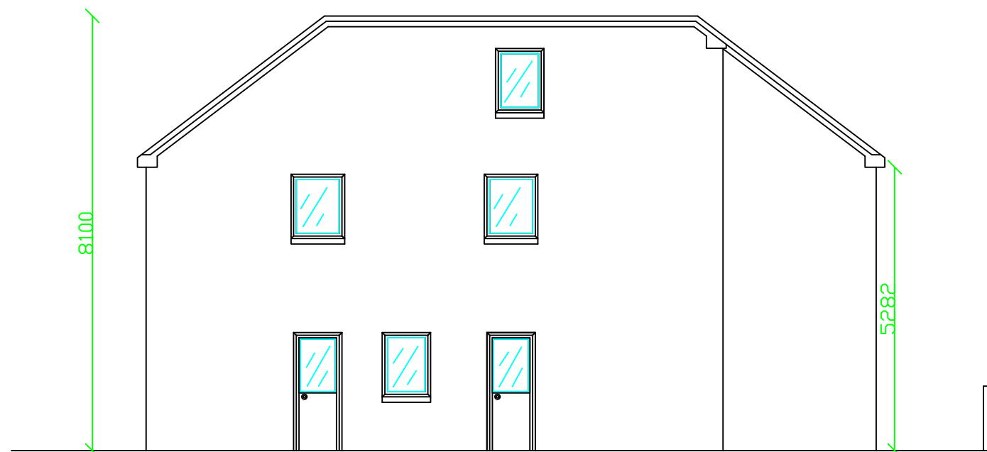
SOUTH ELEVATION
